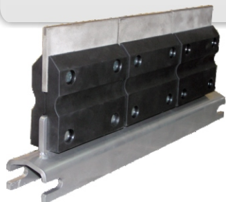
Blade Cartridge Allows for easy change out of scraper blades from either side of the conveyor.
